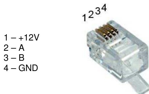
Slika 5. Raspored pinova
